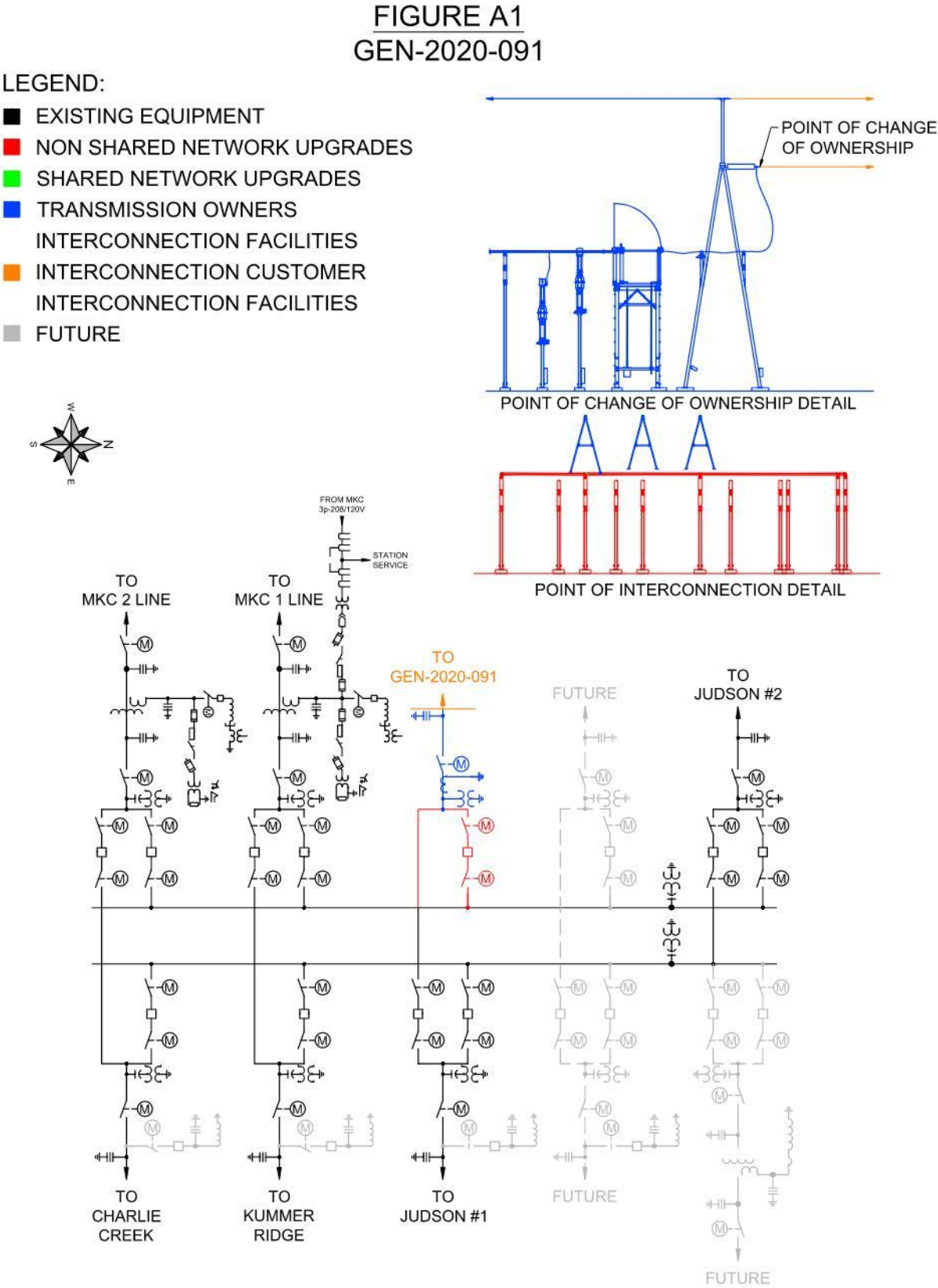
Figure A1: Proposed Switching Diagram
